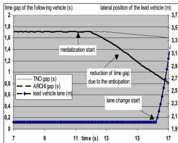
Figure 3: behaviours using a car following law versus ARCHISIM behavioural model
