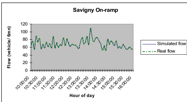
Figure 5: simulated flow for one on-ramp
