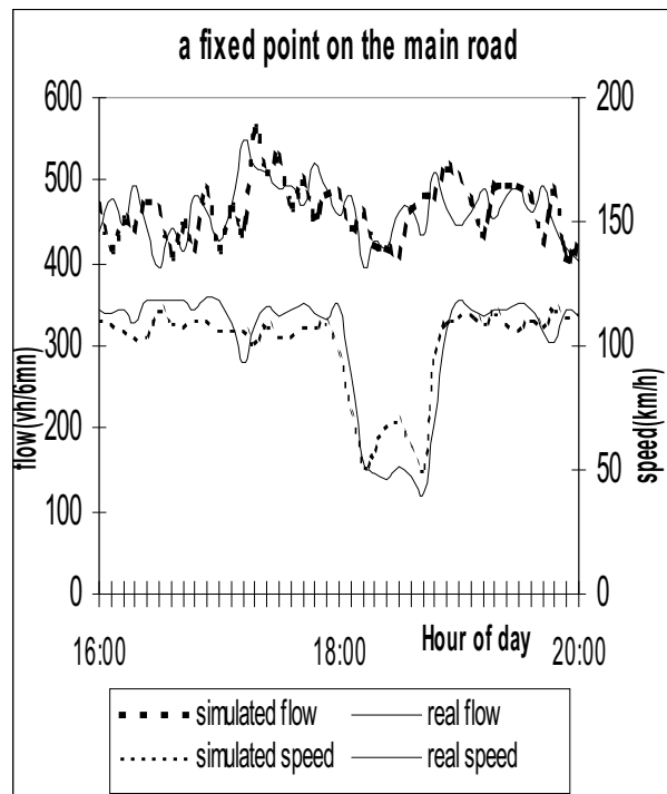
Figure 7: results on the main motorway including a peak hour
