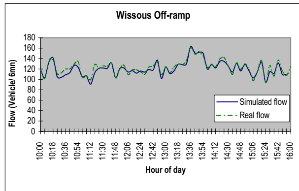
Figure 6: simulated flow for one off-ramp
