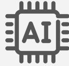
Artificial Intelligence
